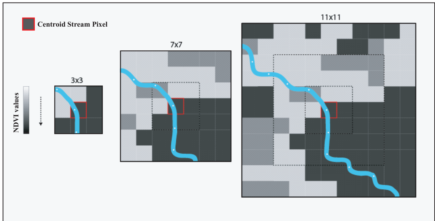
Figure 4. Schematic diagram illustrating a sample of the kernel analysis used in this study. The centroid stream pixel (outlined in red) is attributed with values that represent the statistics of NDVI for all the surrounding pixels in the kernel window. As the kernel size increases, more pixels are evaluated in the analysis and the resulting values represent a larger extent of the watershed.
