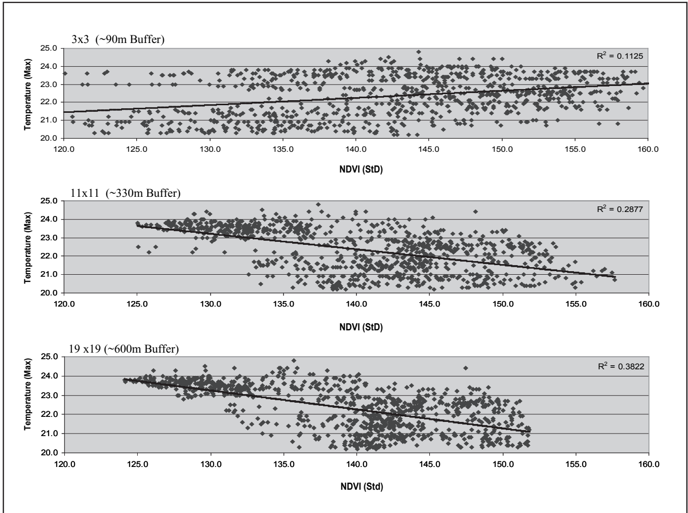
Figure 5. Results of pair-wise regression for kernel analysis showing the standard deviation in NDVI in NDVI pixels against the maximum temperature value for each pixel. Note how the coefficient of determination (r-squared) increases with increasing kernel size, indicating that the regression equation explains more of the variance in temperature as the kernel is increased.
