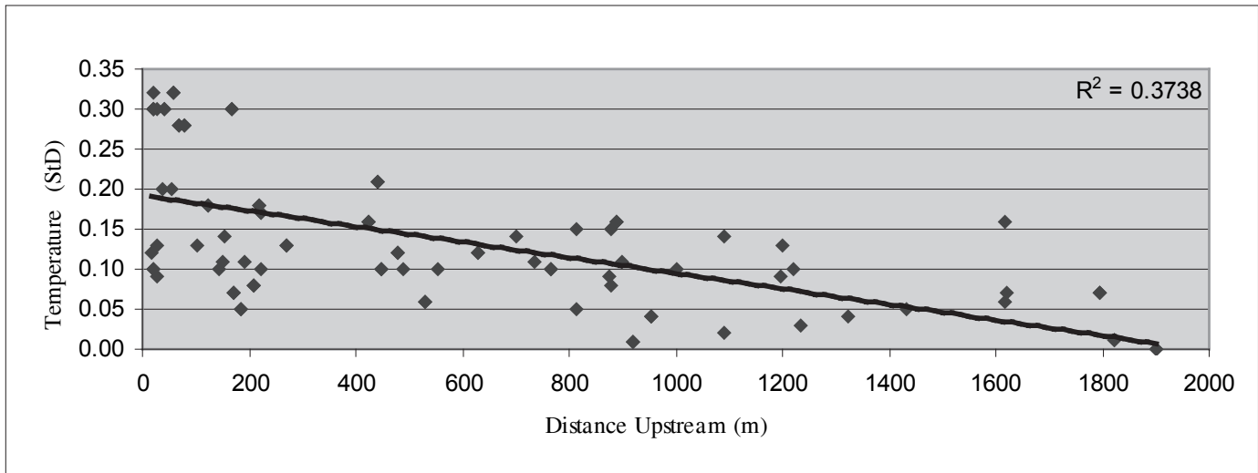
Figure 6. Preliminary pair-wise correlation results for geospatial analysis of water diversion, withdrawal and pump data as they relate to in-stream temperature. Nearly 38% of the variance in downstream water temperatures can be explained by the presence and proximity of a water diversion, pump or withdrawal structure.
